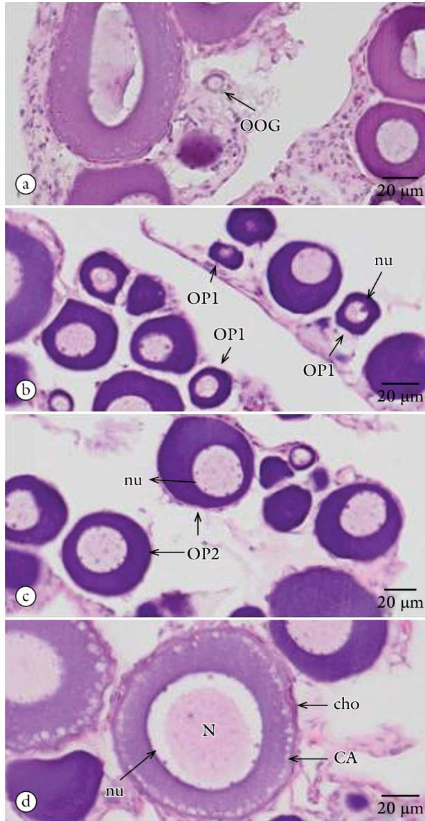
Figure 3. Oocytes at previtellogenic phase (OMS I dan OMS II), (a) oogonia, (b) early perinuclear oocyte, (c) late perinuclear oocyte, (d) cortical alveoli oocyte with choriolamellar layers (1 scale bar = 20 µm).
