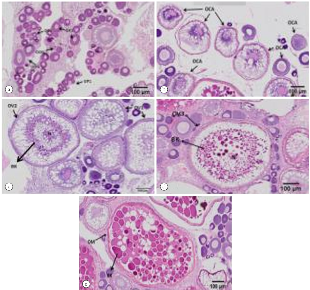
Figure 2. Hystology of M. boosemani rainbowfish ovaries, (a) Hystology of ovary at OMS I, (b) Hystology of ovary at OMS II, (c) Hystology of ovary at OMS III, (d) Hystology of ovary at OMS IV, (e) Hystology of ovary at OMS V (1 scale bar = 100 μm).
